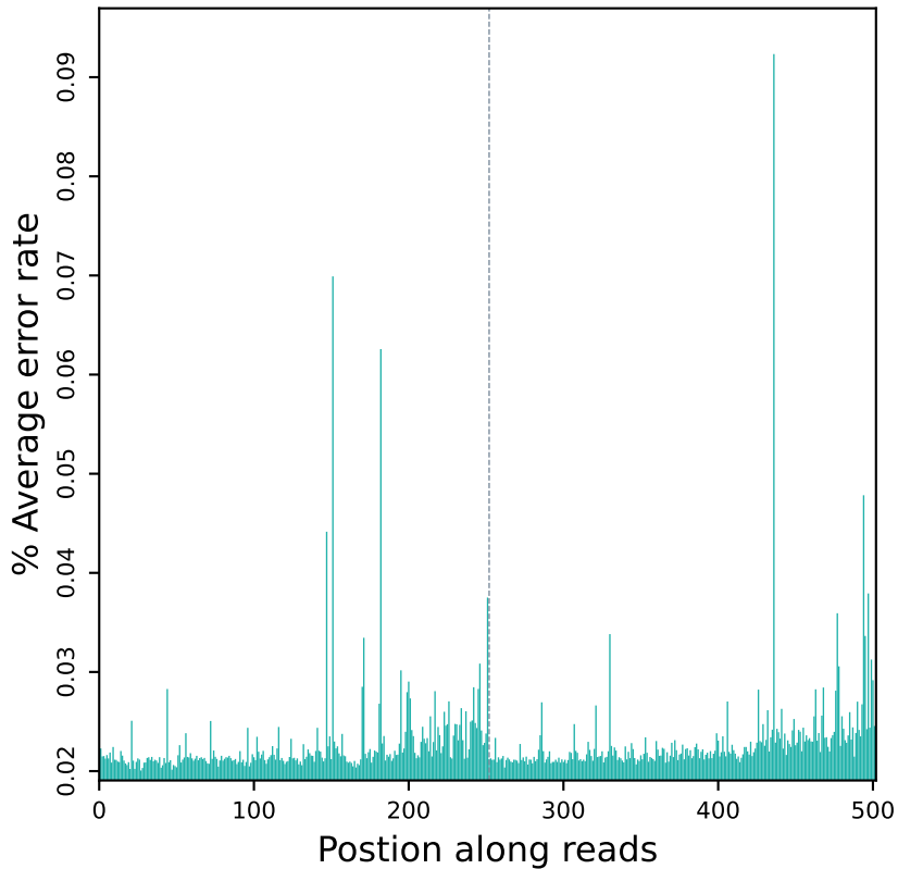
Error rate distribution along reads (R10726)
